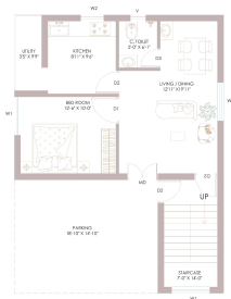
GROUND FLOOR AREA : 1000 SFT.
